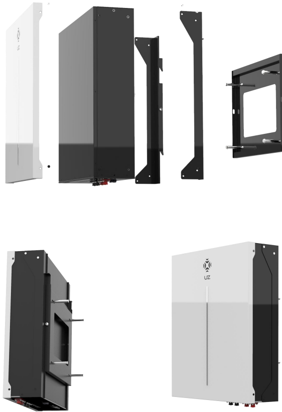
Figure 3、 The vertical installation Parts Appearance Diagram
